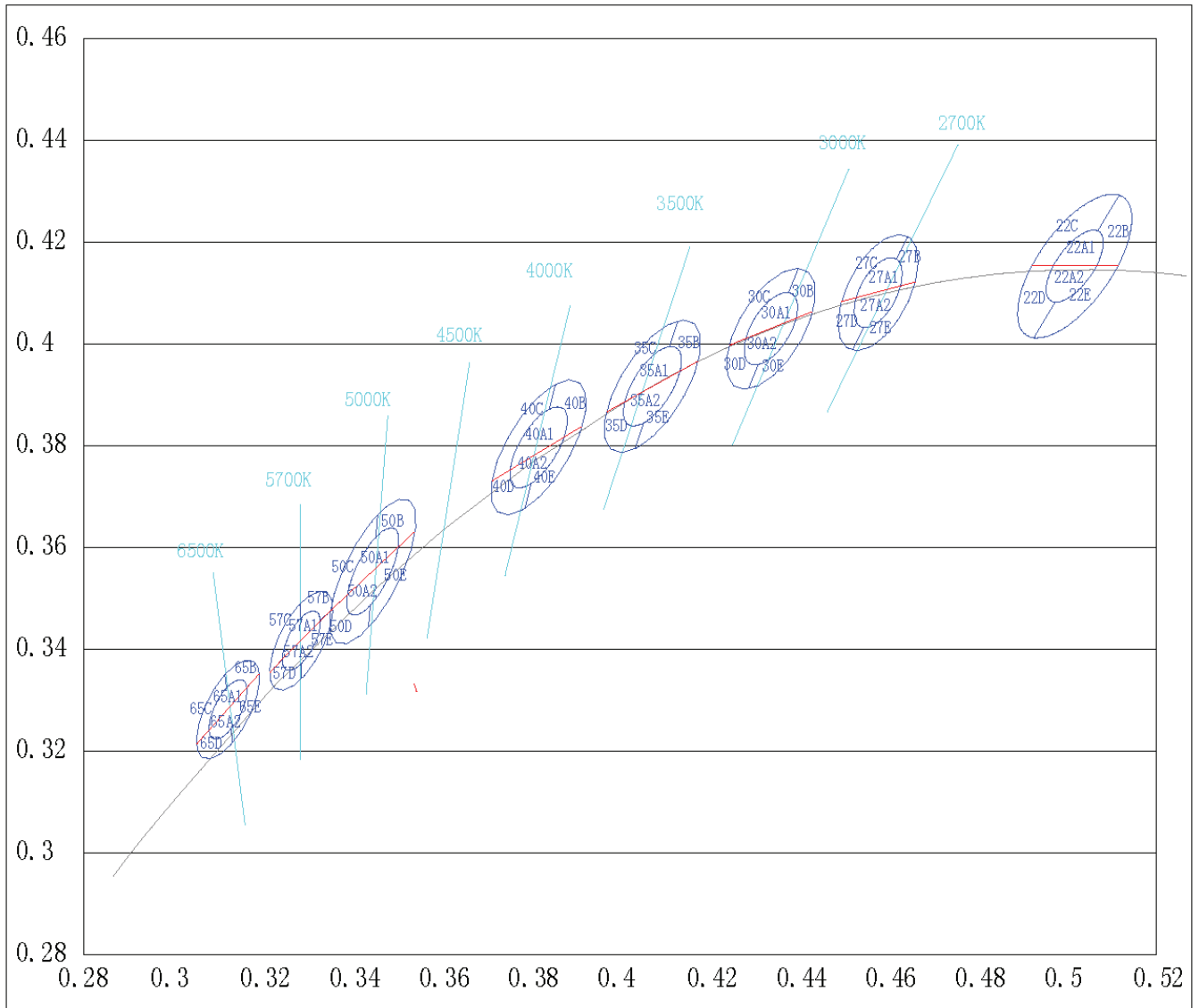
Correlated color temperature bin definitions for 2835R Series at rated current, T_a=25^\circ\text{C}
