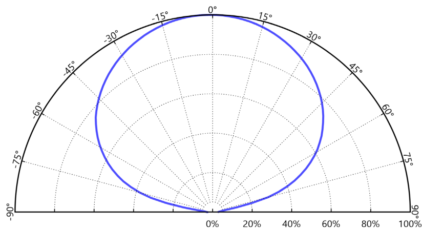
Figure 5b. Typical polar radiation pattern for LUXEON HL4X at 1400mA, T_j=85^{\circ}\text{C}
